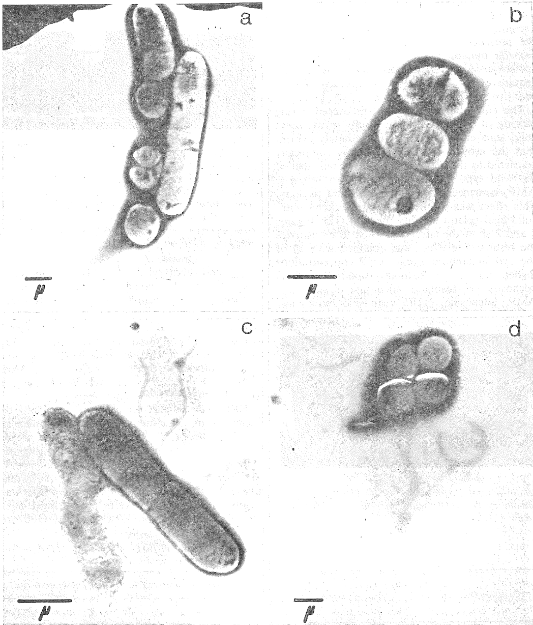
FIG. 3: Electron micrographs of E. coli GPI (negative stain). (a and b) Grown without cyclic AMP; (c and d) grown with 1 \text{ mM} cyclic AMP.
